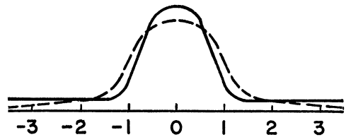
Standardized Variable
